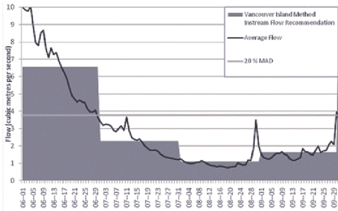
FIGURE 1d Chemainus River June 1 to October 1, Showing Instream Flow Recommendation From Vancouver Island Method,
