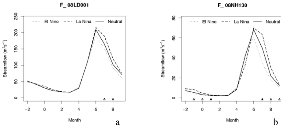
Figure 3.3.4 – Composite analysis results for ENSO on seasonal pattern of mean monthly streamflow ( m^3/s ) a) Adams River - Interior (nival/glacial), and b) Fry Creek - Columbia (nival-glacial). The grey and black triangles indicate significant differences at the 95% and 99% confidence levels respectively. The y-axis shows average streamflow ( m^3/s ) for a given month for the El Niño, La Niña, or Neutral years and the x-axis gives the numeric month (i.e. -2 = October, 0 = December, 8 = August). Source: RHBN data, PCIC.
