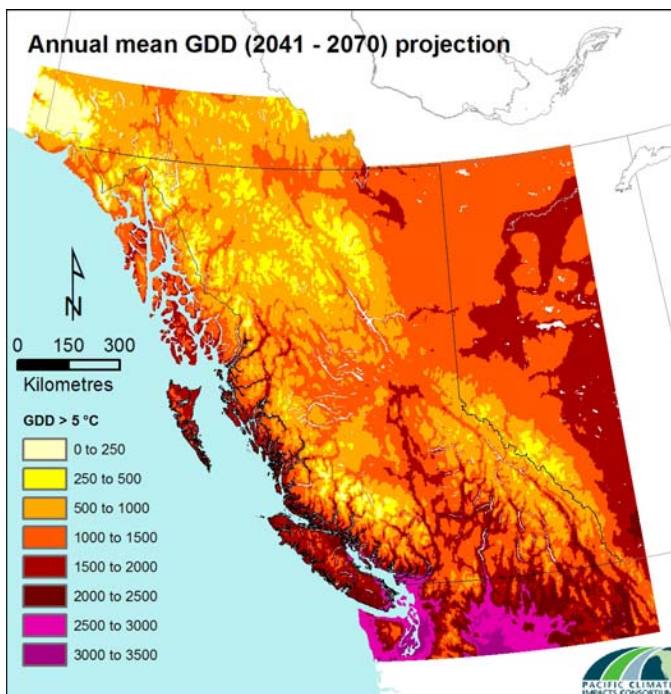
Figure 4.3.4 – 2050s (2041- 2070) high-resolution climate projection of mean annual growing degree days using downscaled temperature with PRISM climatology delta method with CGCM3 following A2 emissions scenario. Source: LLNL (IPCC AR4) data, ClimateBC.
