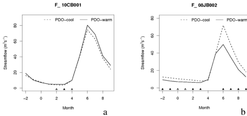
Figure 3.3.7 – Composite analysis results for PDO on seasonal pattern of mean monthly streamflow (m 3 /s) a) Sikanni Chief – Peace Basin (nival) and b) Stellako River – Interior (nival/glacial). The grey and black triangles indicate significant differences at the 95% and 99% confidence levels respectively. The y-axis shows average streamflow (m 3 /s) for a given month for the PDO cool and PDO warm phases and the x-axis gives the numeric month (i.e. -2 = October, 0 = December, 8 = August). Source: RHBN data, PCIC.
