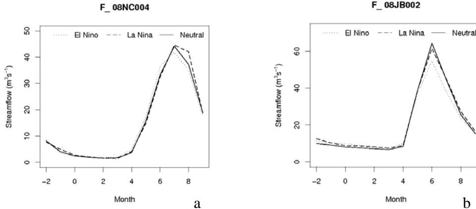
Figure 3.3.5 – Composite analysis results for ENSO on seasonal pattern of mean monthly streamflow ( m^3/s ) a) Canoe River - Columbia (nival/glacial), and b) the Stellako River – Interior (nival/glacial). The grey and black triangles indicate significant differences at the 95% and 99% confidence levels respectively. The y-axis shows average streamflow ( m^3/s ) for a given month for the El Niño, La Niña, or Neutral years and the x-axis gives the numeric month (i.e. -2 = October, 0 = December, 8 = August). Source: RHBN data, PCIC.
