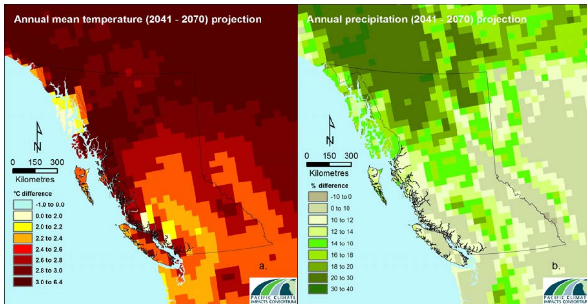
Figure 4.2.1 – 2050s (2041-2070) climate anomaly projections from CRCM4 forced with CGCM3 and A2 emissions scenario (a) annual mean temperature, and (b) annual precipitation. Source: Ouranos Consortium data.
