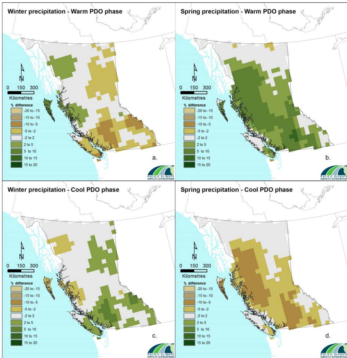
Figure 2.2.5 – Seasonal climate variability for precipitation (a) warm PDO phase winter, (b) warm PDO phase spring, (c) cool PDO phase winter and (d) cool PDO phase spring for British Columbia. Results are based on 1900 to 2004 (ENSO) and calculated as a difference from the long-term average, percent of the 1961 – 1990 climatology. Source: CANGRID (50 km) data.
