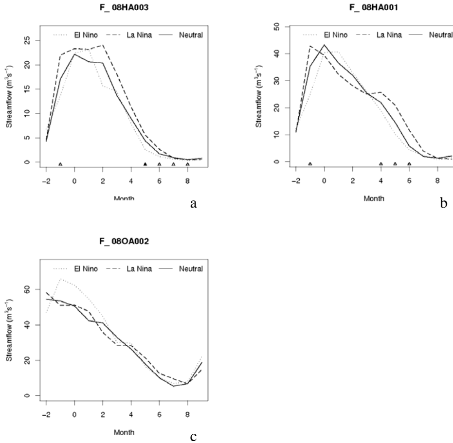
Figure 3.3.3 – Composite analysis results for ENSO on seasonal pattern of mean monthly streamflow ( m^3/s ) for the South Coast a) Koksilah River (pluvial), b) Chemainus River (nival-supported pluvial), and on the North Coast c) Yakoun River (pluvial). The grey and black triangles indicate significant differences at the 95% and 99% confidence levels respectively. The y-axis shows average streamflow ( m^3/s ) for a given month for the El Niño, La Niña, or Neutral years and the x-axis gives the numeric month (i.e. -2 = October, 0 = December, 8 = August). Source: RHBN data, PCIC.
