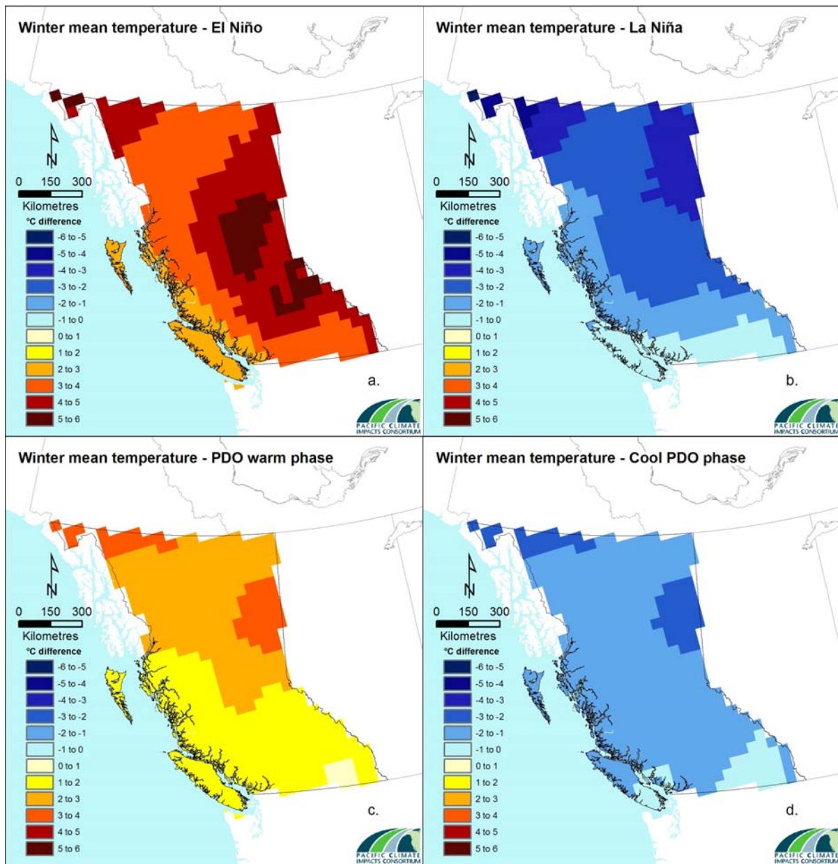
Figure 2.2.3 – Seasonal climate variability for mean temperature (a) El Niño, (b) La Niña, (c) warm PDO phase and (d) cool PDO phase for British Columbia. Results are composites from the 1900-2004 (ENSO) and 1900-1998 (PDO) and calculated as degree Celsius difference from the long-term average. Source: CANGRID (50 km) data.
