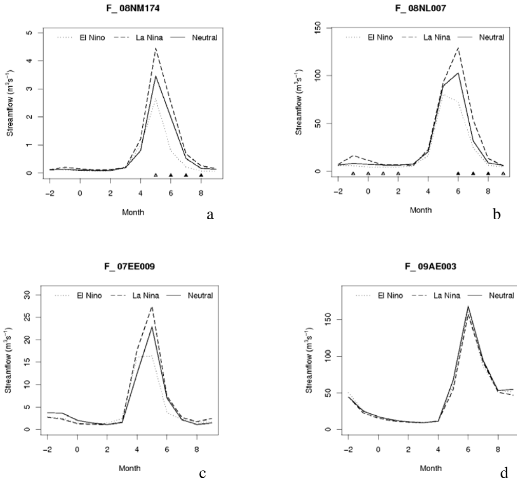
Figure 3.3.2 – Composite analysis results for ENSO on seasonal pattern of mean monthly streamflow (m 3 /s) for the a) West Kettle River – Okanagan (nival), b) Similkameen River (at Princeton) – Okanagan (nival/hybrid), c) Chuchinka Creek - Peace Basin (hybrid), and d) Swift River - Northwest (nival). The grey and black triangles indicate significant differences at the 95% and 99% confidence levels respectively. The y-axis shows average streamflow (m 3 /s) for a given month for the El Niño, La Niña, or Neutral years and the x-axis gives the numeric month (i.e. -2 = October, 0 = December, 8 = August). Source: RHBN data, PCIC.
