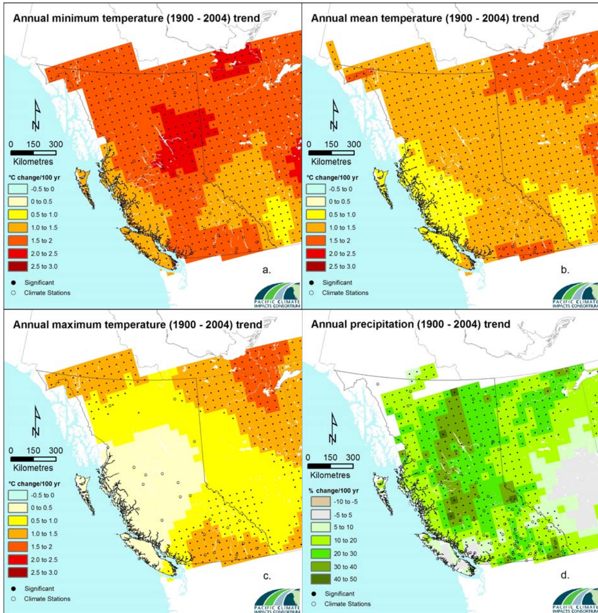
Figure 2.1.1 – Annual trends in (a) minimum, (b) mean, (c) maximum temperature and (d) precipitation for British Columbia. Results are based on 1900 to 2004 data and calculated as degree Celsius change per century. Black solid circles indicate statistically significant results (95% confidence level). Open circles show the location of Adjusted Historical Canadian Climate Station sites (AHCCD). Source: CANGRID (50 km) data; adapted from Zhang et al. 2000.
