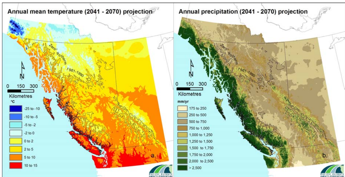
Figure 4.3.2 – 2050s (2041-2070) high-resolution climate projections using PRISM climatology delta-method using HadCM3 B1 emissions scenario (a) annual mean temperature, (b) annual precipitation. Source: LLNL (IPCC AR4) data, ClimateBC.
