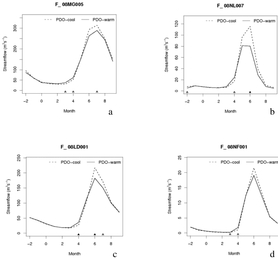
Figure 3.3.6 – Composite analysis results for PDO on seasonal pattern of mean monthly streamflow (m 3 /s) a) Lillooet River - South Coast (nival/glacial), b) Similkameen River - Okanagan (nival/hybrid), c) Adams River – Interior (nival/glacial), and d) Kootney River – Columbia (nival/glacial). The grey and black triangles indicate significant differences at the 95% and 99% confidence levels respectively. The y-axis shows average streamflow (m 3 /s) for a given month for the PDO cool and PDO warm phases and the x-axis gives the numeric month (i.e. -2 = October, 0 = December, 8 = August). Source: RHBN data, PCIC.
