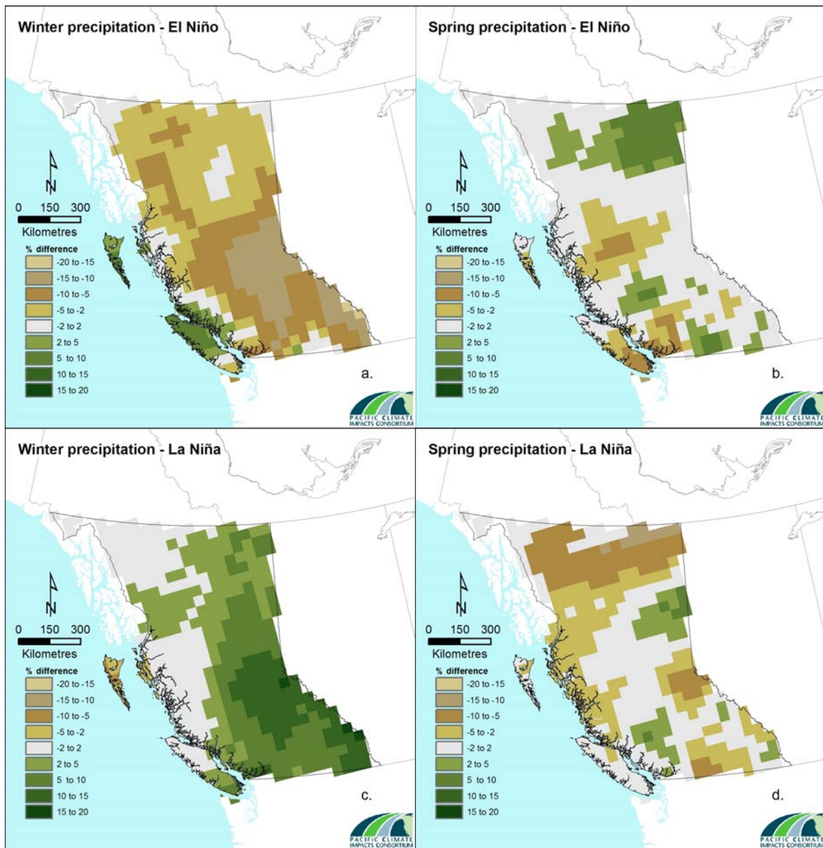
Figure 2.2.4 – Seasonal climate variability for precipitation (a) El Niño winter, (b) El Niño spring, (c) La Niña winter and (d) La Niña spring for British Columbia. Results are based on 1900 to 2004 (ENSO) and calculated as a difference from the long-term average, percent of the 1961 – 1990 climatology. Source: CANGRID (50 km) data.
