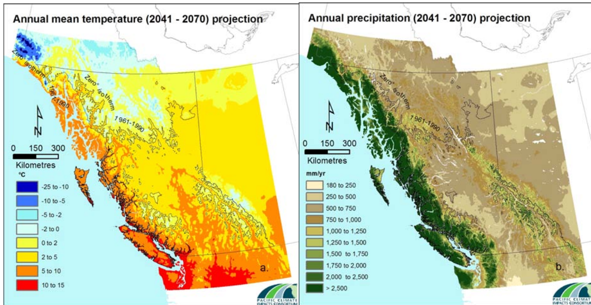
Figure 4.3.1 – 2050s (2041-2070) high-resolution climate projections using PRISM climatology delta-method using CGCM3 A2 emissions scenario (a) annual mean temperature, (b) annual precipitation. Source: LLNL (IPCC AR4) data, ClimateBC.
